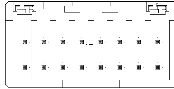
16POS(X-KEY):KF7025-0816-2.5DIP
